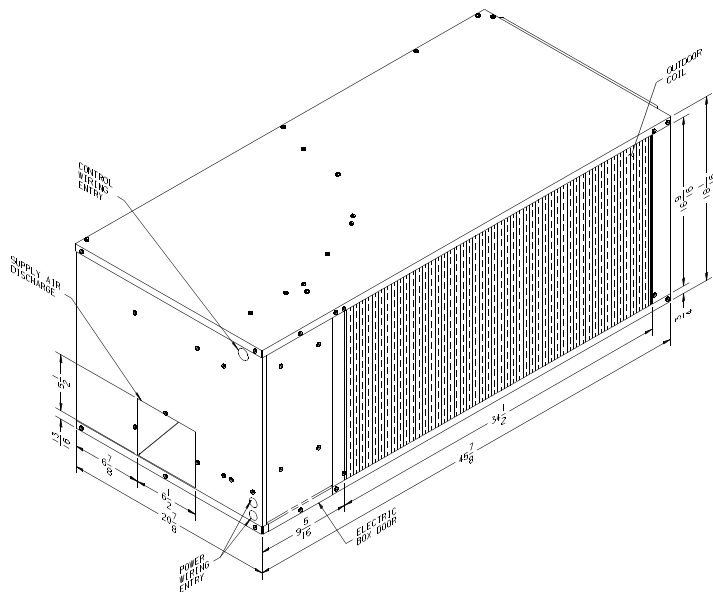
FIGURE 1 (Left Hand Configuration)
