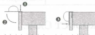
"Top-of-Dock" Installation Method
