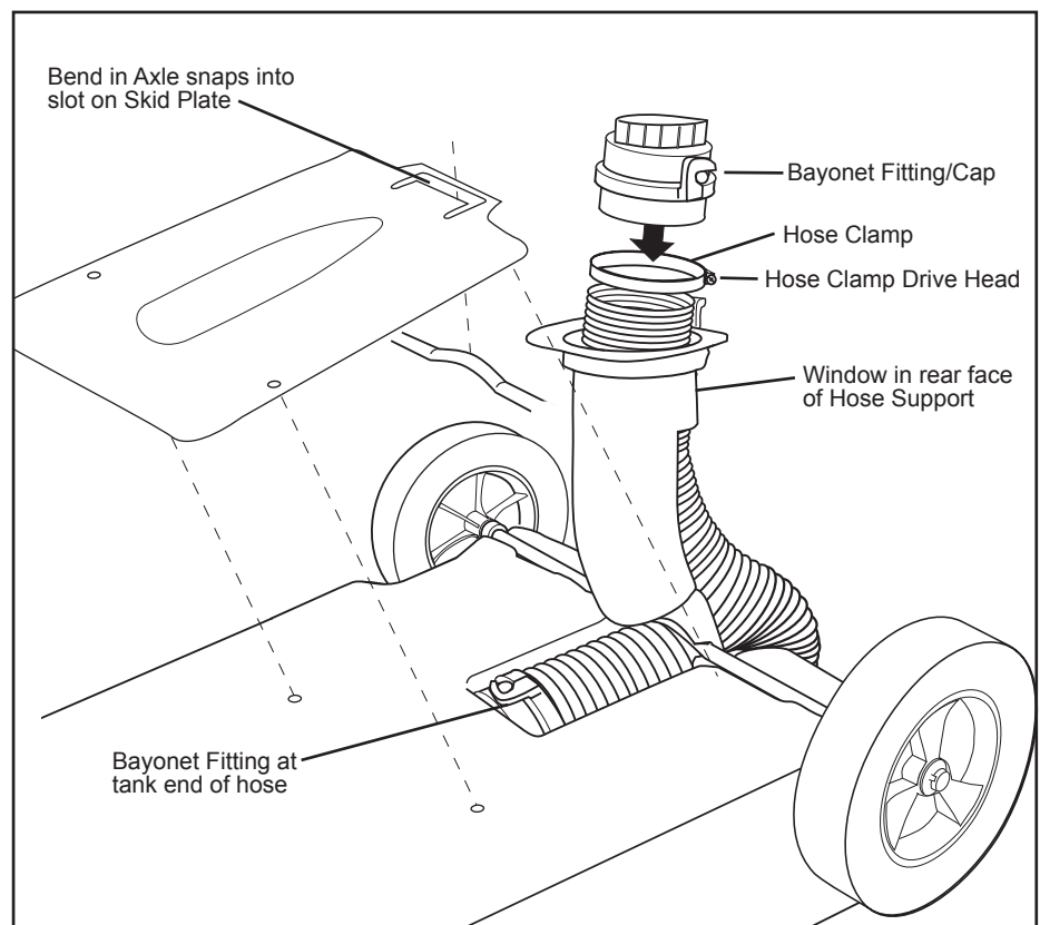
Fig. A Hose Support and Tank component assembly
