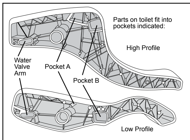
FIGURE 3 - PEDAL REATTACHMENT
