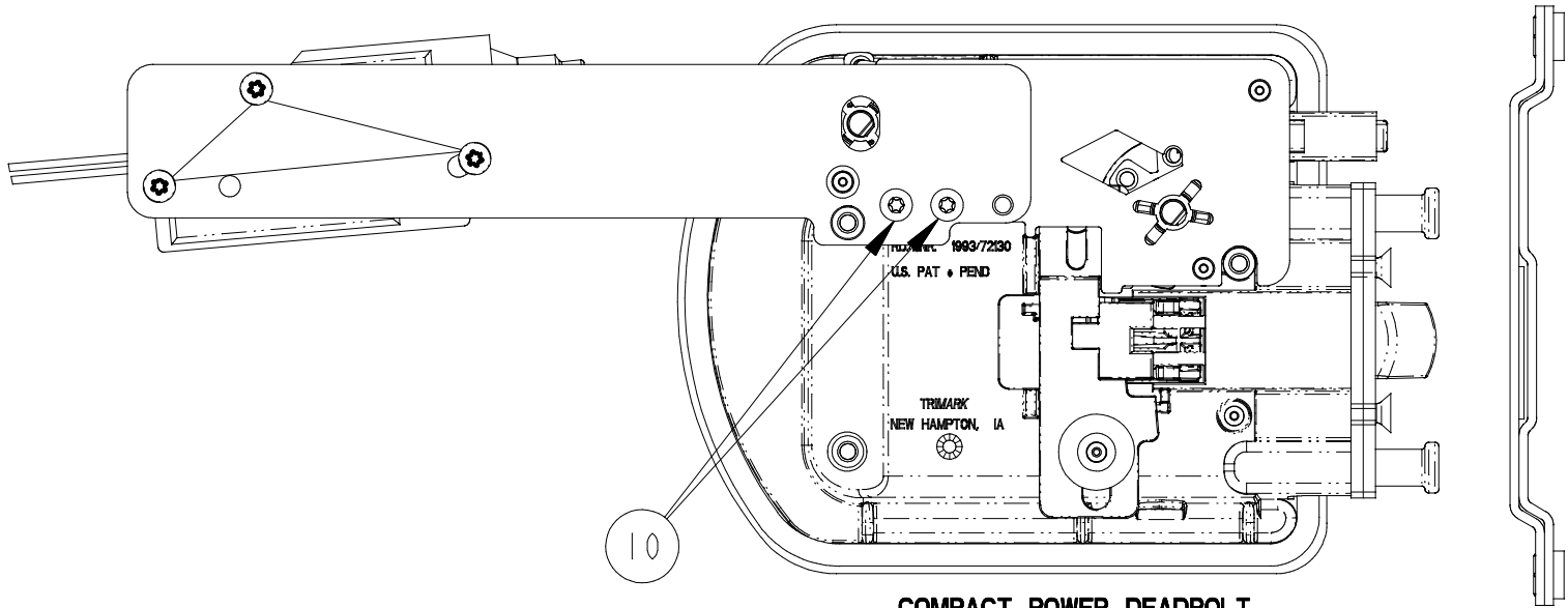
COMPACT POWER DEADBOLT (INSIDE HANDLE ASSEMBLY NOT SHOWN FOR CLARITY)
