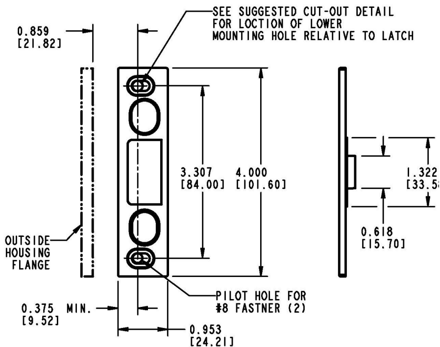
DIE CAST STRIKER PLATE FOR STANDARD VERSION
