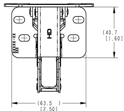
Alternate Mounting
