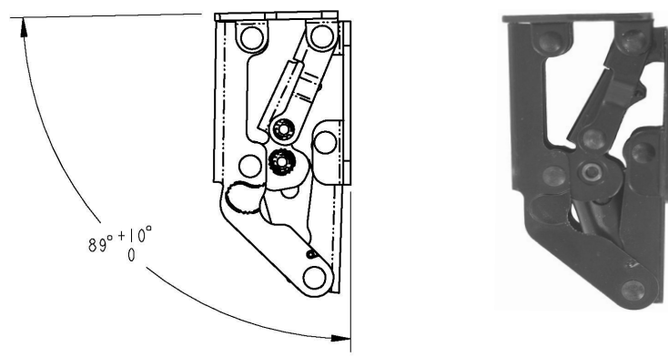
Hinge Closed
