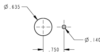
RECOMMENDED MOUNTING
