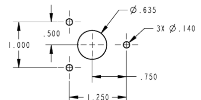
(OPTIONAL MOUNTING)
