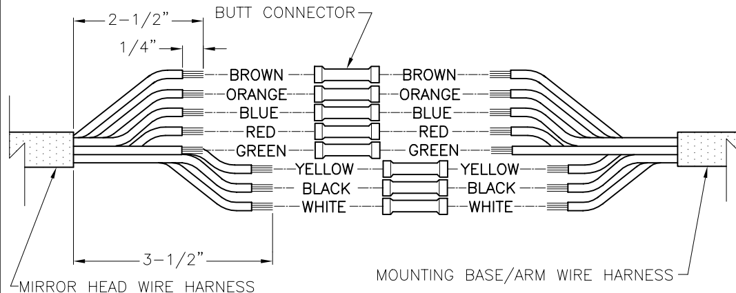
VIEW B-B
