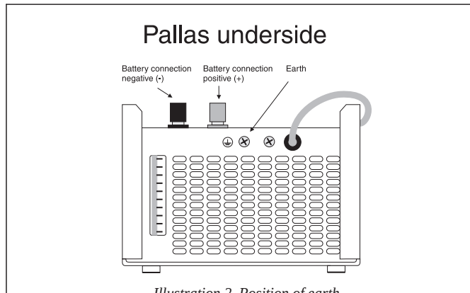
Illustration 2. Position of earthing screw on the Pallas 12/25
