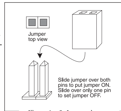
Illustration 9. Jumper placement.
