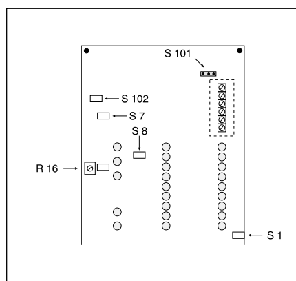
Illustration 7. Adjusting the maximum charge current.
