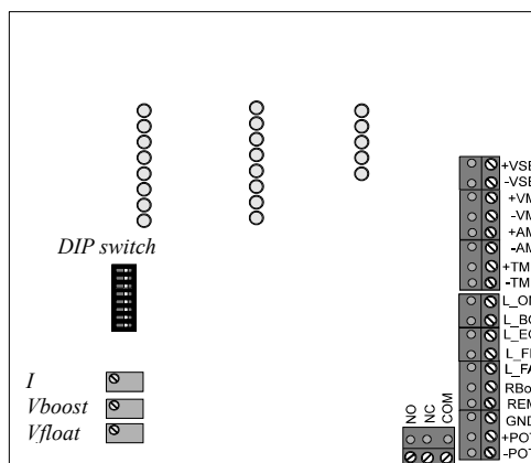
Illustration 7. Location of the DIP-switch and potentiometers.
