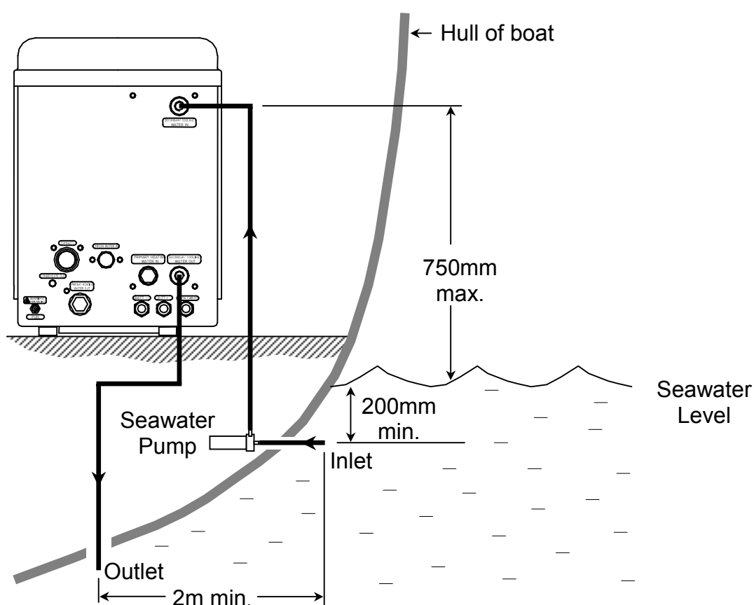
Figure 4: Plumbing the secondary coolant circuit – marine systems
