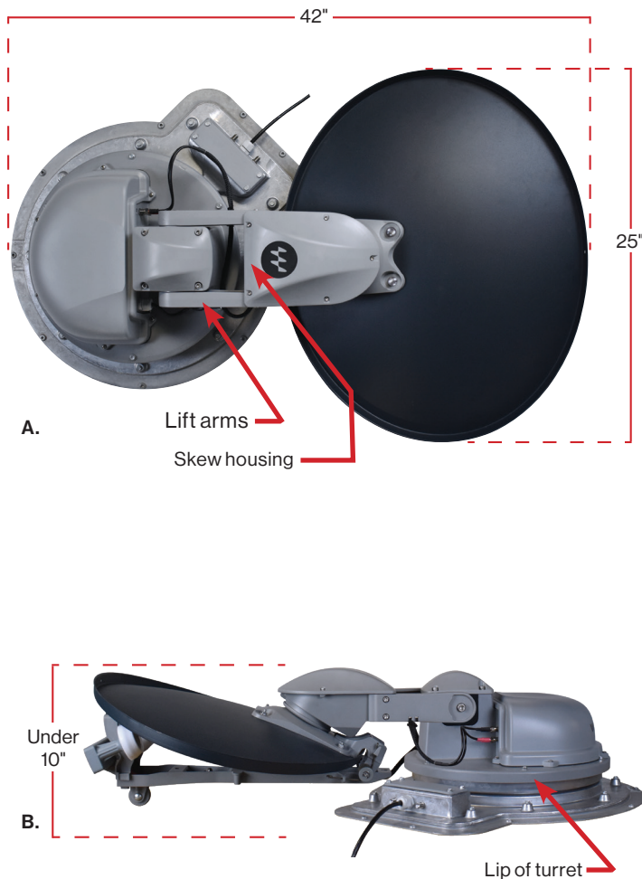
FIGURE 1.A. Dimensions of SK2DISH B. Stowed A,B. Location of skew housing, lift arms, and lip at the base of the turret
