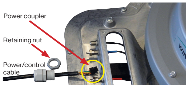
FIGURE 13. Power coupler unclipped
