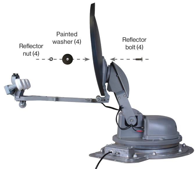
FIGURE 10. Attach reflector with 4 bolts (back of reflector), washers and nuts (front of reflector)
