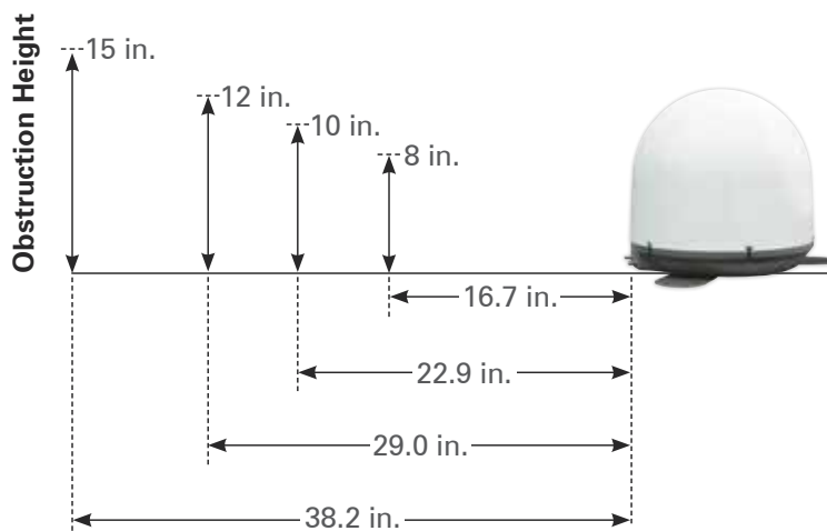
Min. Distance to be Maintained from Antenna
