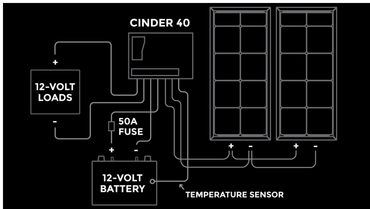
Figure 5: 12-Volt Installation Diagram
