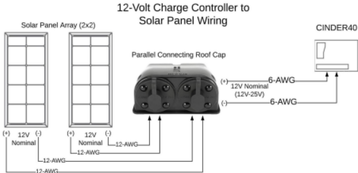
Figure 6: 12-Volt Charge Controller to Solar Panel Wiring example
