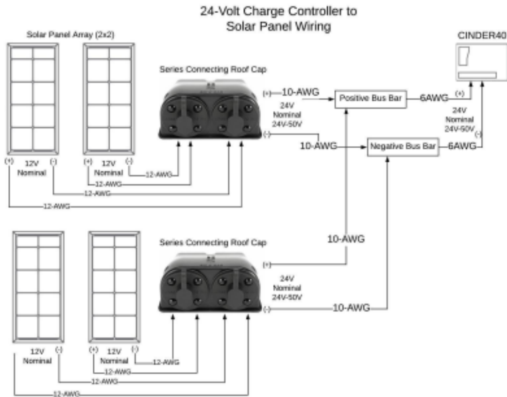
Figure 8: 24-Volt Charge Controller to Solar Panel Wiring example
